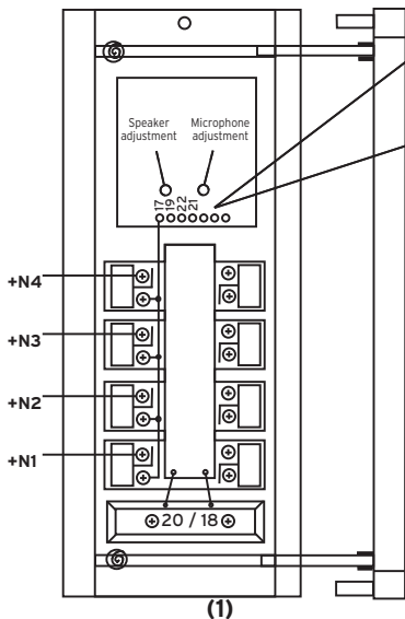
Figure-1 shows 4-apartment outdoor panel. outputs +N1,+N2,+N3,+N4 must be connected to doorphones' terminal seperately. Minimum tickness is 0.50mm
